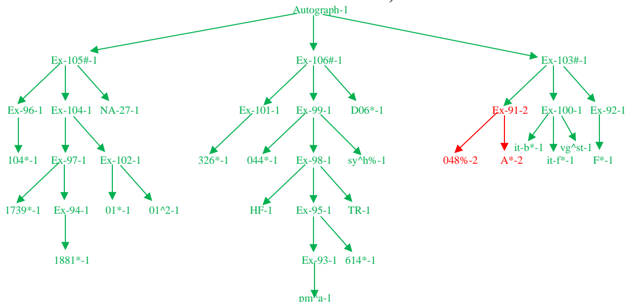
Figure 4.9 Distribution of 1:6,2
