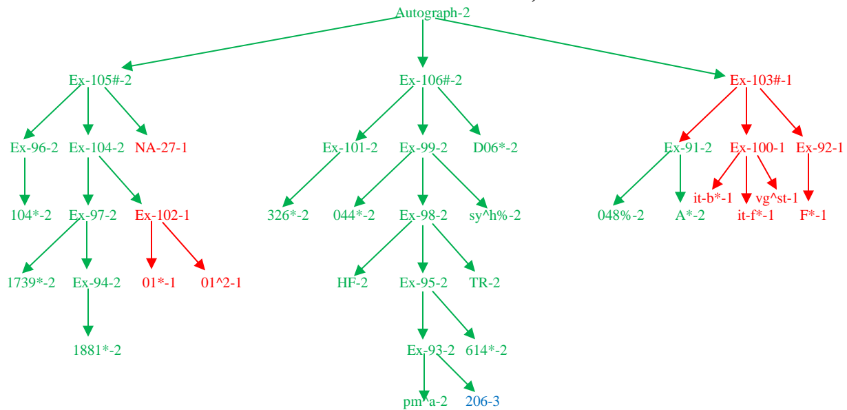
Figure 4.6 Distribution of 2:14,1
