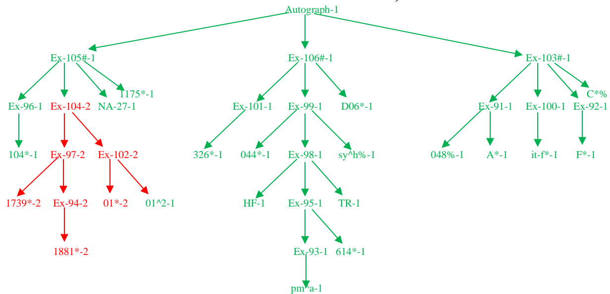
Figure 4.3 Distribution of 4:21,1
