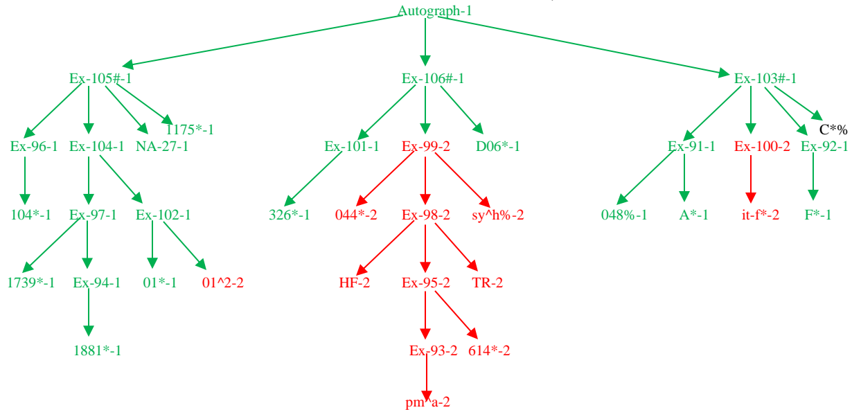
Figure 4.1 Distribution of 2:13,1
